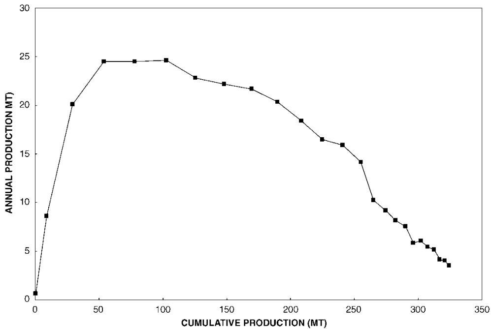
Figure 3. Forties Production, Annual vs. Cumulative
