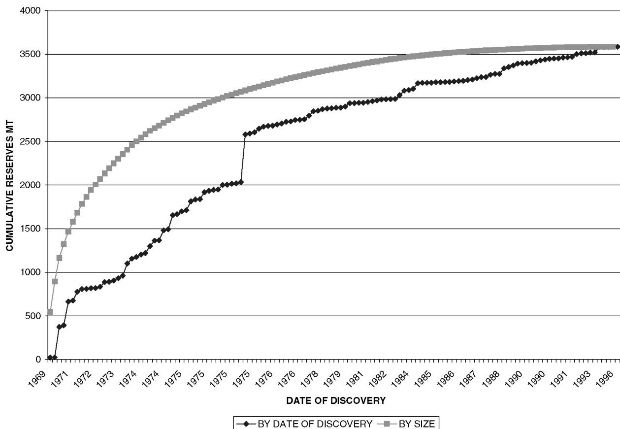
Figure 1. UK Reserves, Ordered by Field Size and by Date of Discovery. Data is from UK Department of Trade and Industry (2001). Developed fields only
