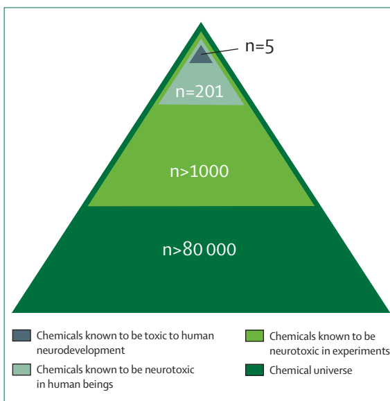
Figure 2: Diagram of the extent of knowledge of neurotoxic chemicals
