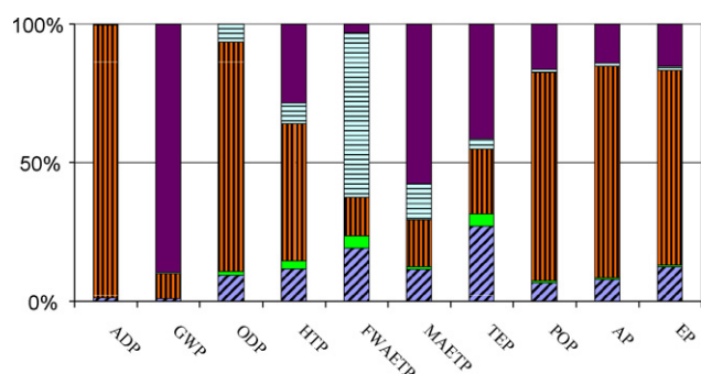
Fig. 6 – Process contribution for case 2: (■) direct emissions; (■) remaining process operation; (■) coal supply operation; (■) remaining infrastructure; (■) coal supply infrastructure.
