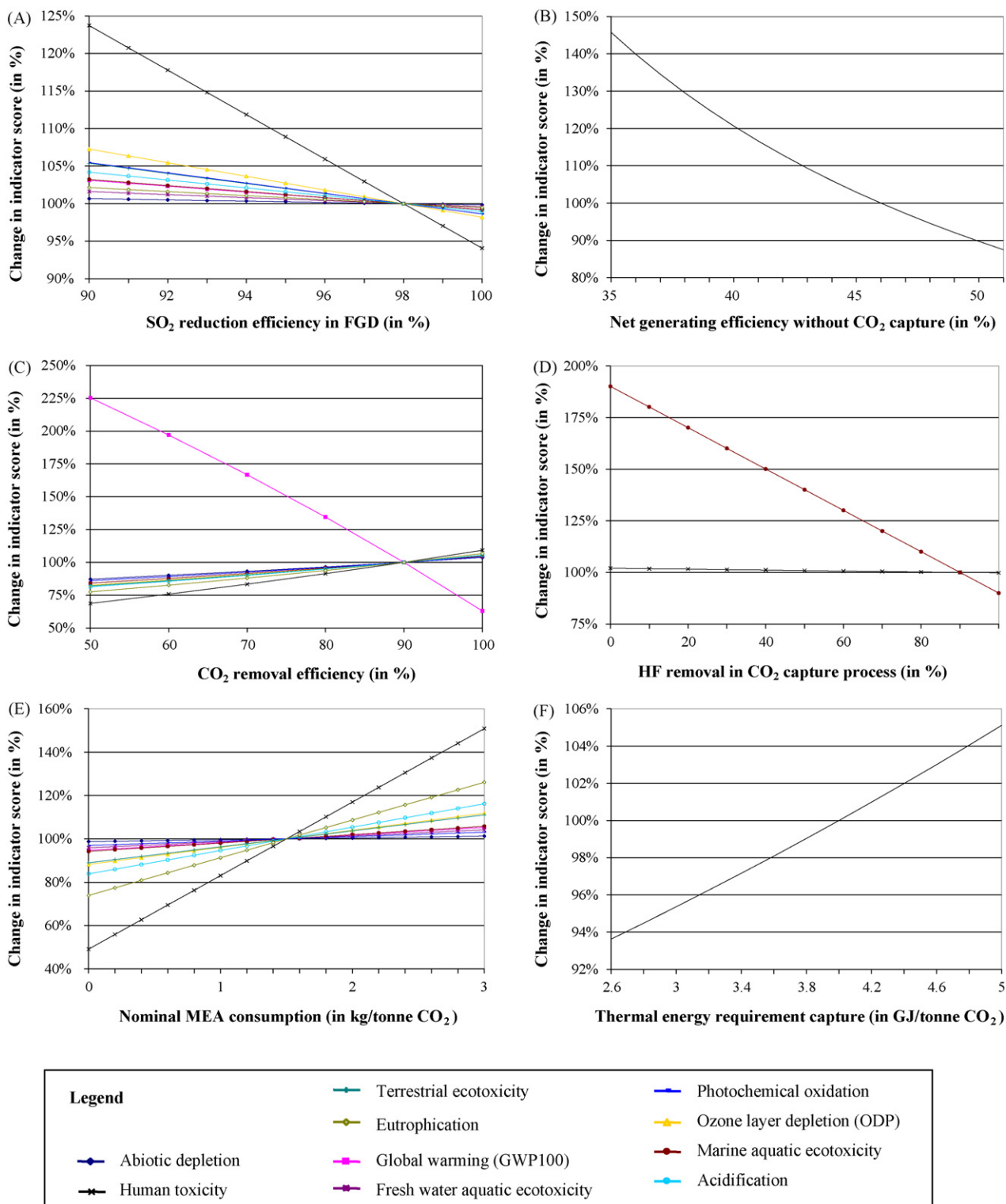
Fig. 9 – Sensitivity analyses for case 3 for selected parameters. On the x-axes the parameter values are given and on the y-axes the percental change in indicator scores in comparison with the default results for case 3 are presented.
