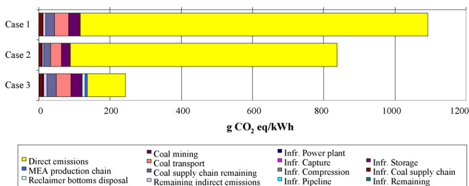
Fig. 4 – Breakdown of global warming potential into first, second and third-order processes for cases 1, 2 and 3.
