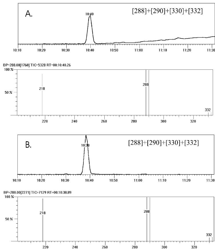
Fig. 2. Ion chromatogram and SIM-spectra from (A) Human milk and (B) Irgasan DP300.
